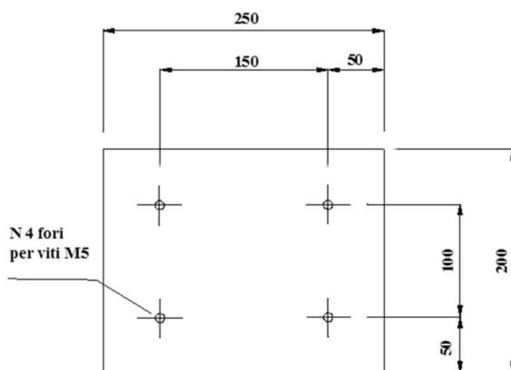
Figure 11 -Maximum dimensions and installation template of RGDAT-A70 for using on MV cells.
