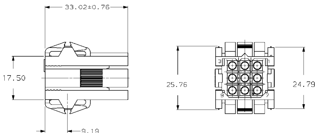
Figure 15 -Rectangular connector (UP side).
