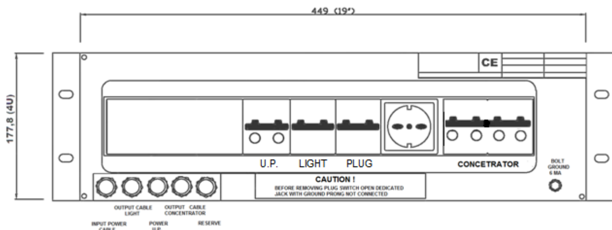
Fig. 4 - Control panel for Auxiliary Service GSCL001/3
