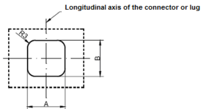
Figure 6 – Tool for compressing the earthing lug
