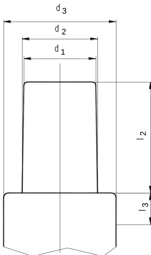
Figure 4 – Interface
