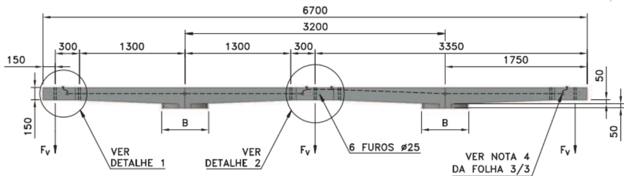
VISTA FRONTAL
