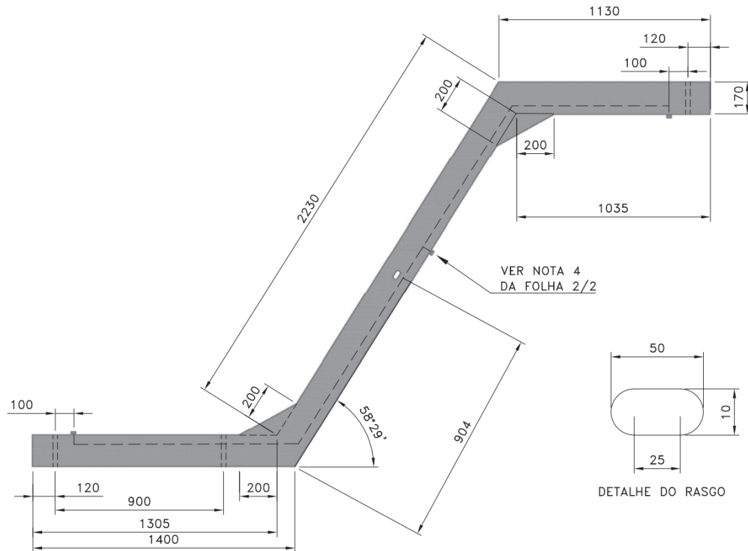
VISTA LATERAL – CRUZETA "Z"
