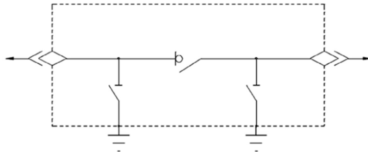
Figure 11. Plug-in switch-disconnector with earthing-switches
