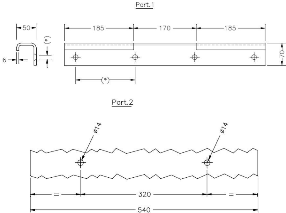
Figure 1. Switchgear coupling support.
