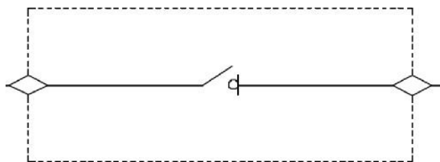
Figure 6. Functional scheme for switch-disconnector for bare conductor lines
