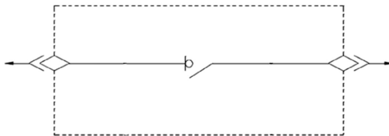
Figure 12. Plug-in switch-disconnector without earthing-switches
