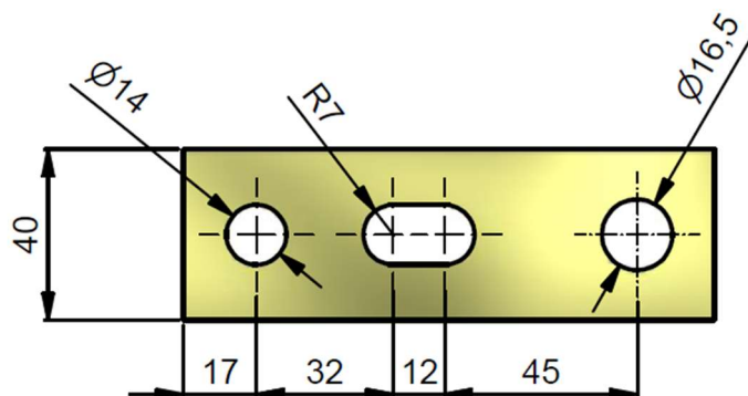
Figure 8. Example of connection plate
