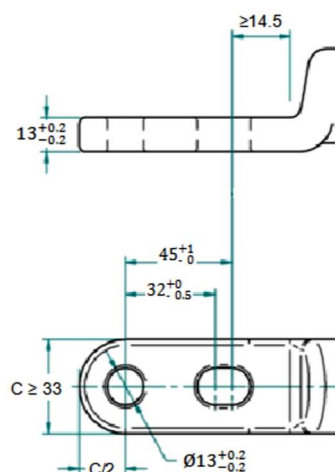
Figure 7. Eyelet terminal
