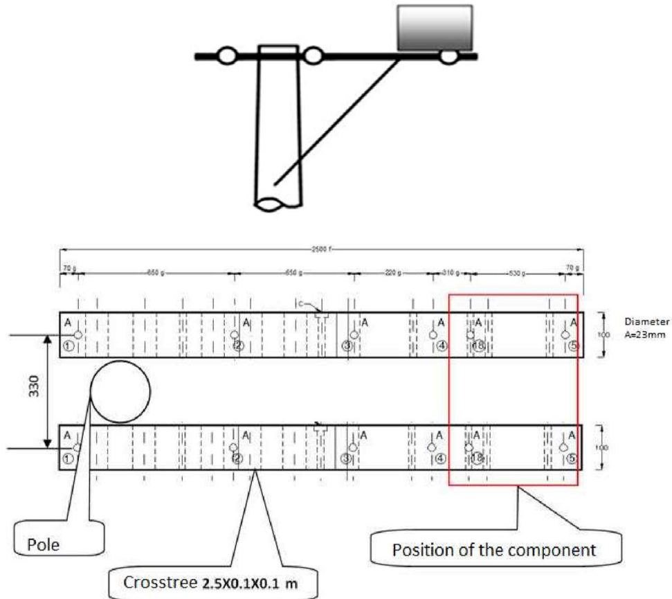
Figure 2. Switchgear in horizontal surface for Colombia
